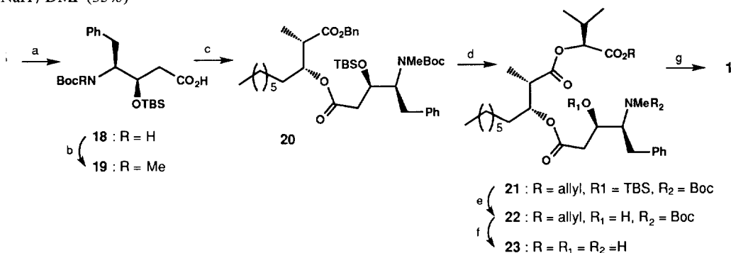
Scheme 3. Reagents: a. i) TBSCl, Imd / DMF (100%); ii) 2M NaOH (84%). b. MeI, NaH / THF (77%). c. 4 , DCC, DMAP / CH 2 Cl 2 (77%). d. i) H 2 , Pd(OH) 2 / EtOH; ii) 8 , DCC, DMAP / CH 2 Cl 2 (96% in two steps). e. HF / pyridine (87%). f. i) (Ph 3 P) 4 Pd, morpholine / THF (97%); ii) TFA / CH 2 Cl 2 (94%); g. DPPA, iPr 2 NEt / DMF (1 mmol/l) (44%).
