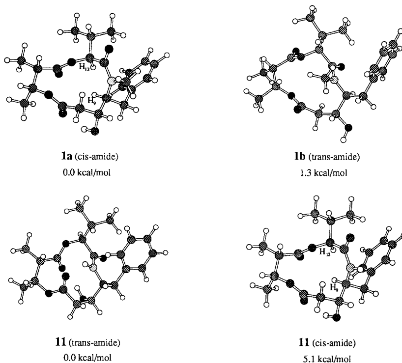
Figure 1. Lowest Energy Conformations of the Cis- and Trans-amides of Hapalosin ( 1 ) and N-Demethylhapalosin ( 11 ) Optimized by MM2* Force Field Calculations.
