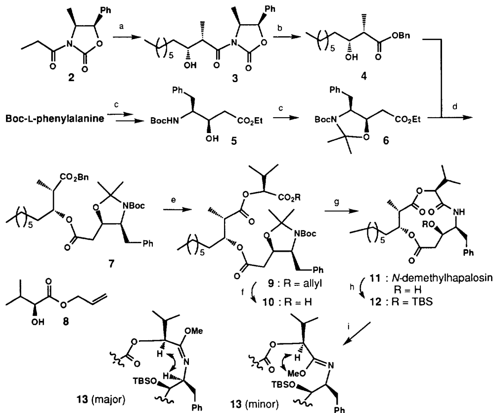
Scheme 1. Reagents: a. Bu 2 BOTf, Et 3 N / CH 2 Cl 2 , then Me(CH 2 ) 6 CHO (90%). b. nBuLi, BnOH / THF (71%). c. ref. 8. d. i) NaOH; ii) 4 , DCC, DMAP / CH 2 Cl 2 (86% in two steps). e. i) H 2 , Pd(OH) 2 / EtOH; ii) 8 , DCC, DMAP/CH 2 Cl 2 (81% in two steps). f. (Ph 3 P) 4 Pd, morpholine/THF (80%). g. i) TFA / CH 2 Cl 2 ; ii) DPPA, iPr 2 NEt / DMF (1 mmol/l) (83% in two steps). h. TBSCl, Imd / DMF (92%). i. Me 3 OBF 4 , Proton Sponge TM / CH 2 Cl 2 (66%).
